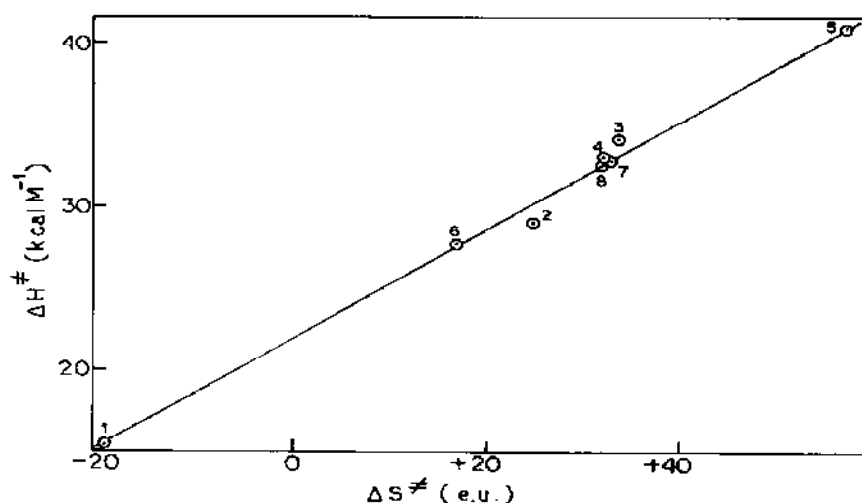
Fig. 2. Isokinetic plot for the water substitution reactions of \text{cis-Co}(\text{NH}_3)_4(\text{OH}_2)_2^{3+} with 1, \text{NO}_2^- ; 2, \text{N}_3^- ; 3, \text{NCS}^- ; 4, \text{Hsal}^- ; 5, \text{Hida}^- ; 6, \text{Hph}^- ; 7, \text{OAc}^- ; 8, \text{Hsucc}^- .
